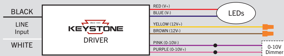
0-10V Dimmer
